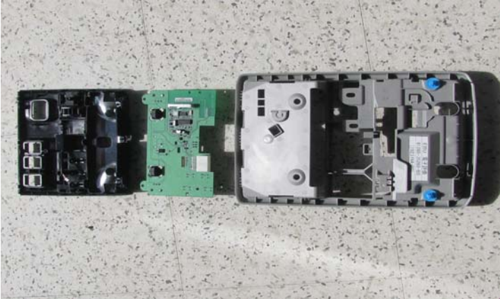
Homelink out of assembly
