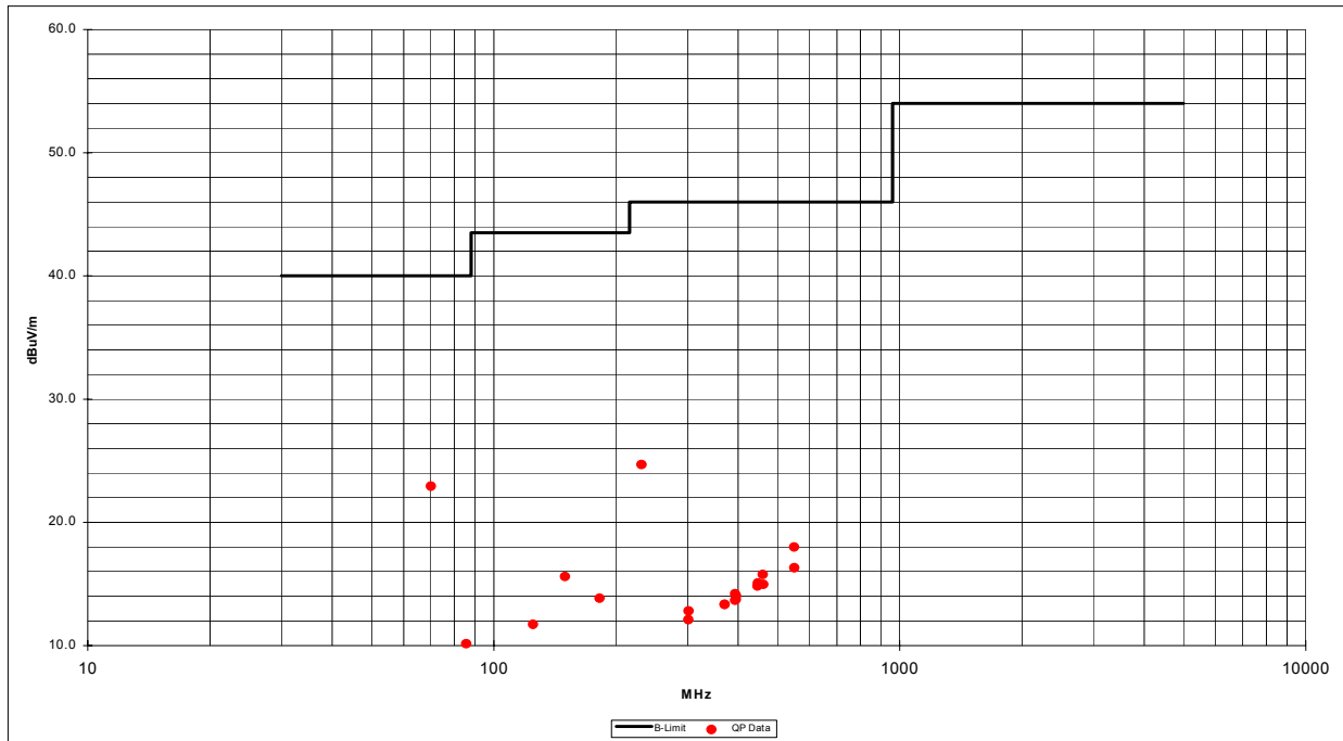
Graph of Quasi-Peak Measurements
