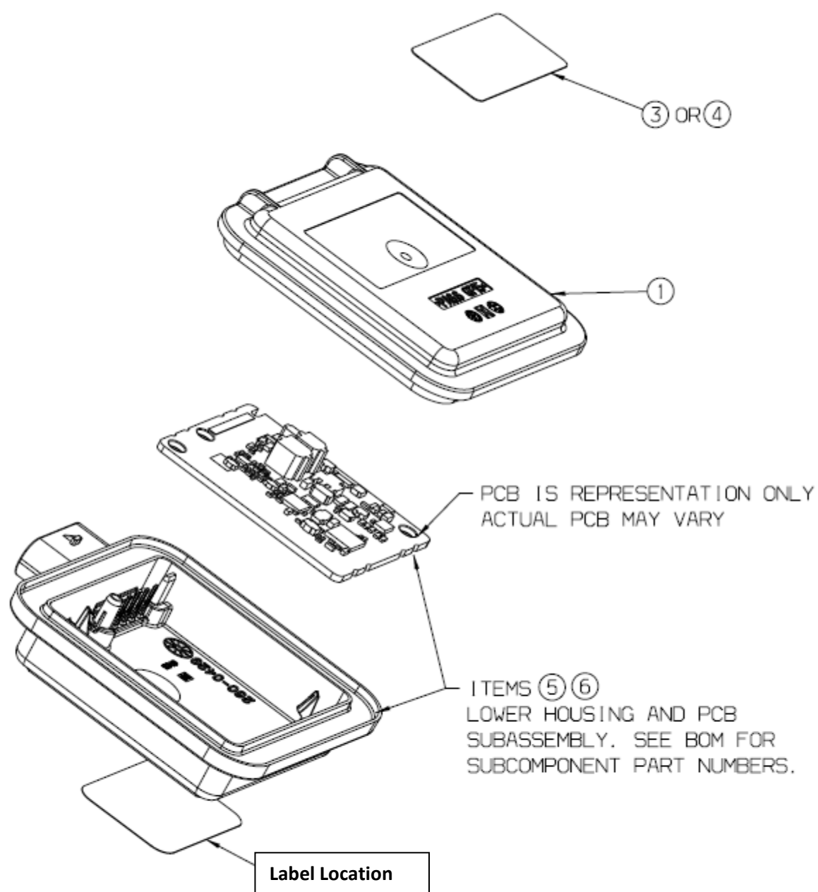
EXPLODED VIEW
