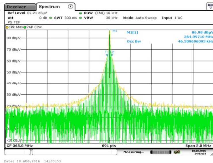
Measuring Occupied Bandwidth at -20dB points20
