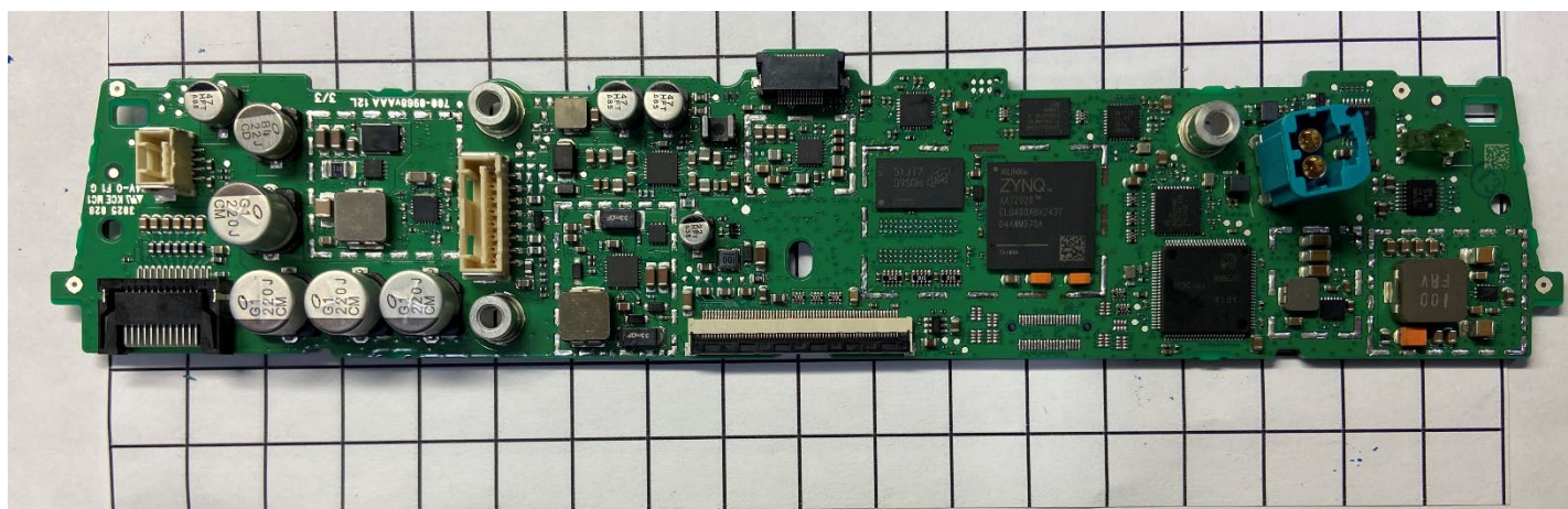
Top Side of PCB with shields removed
