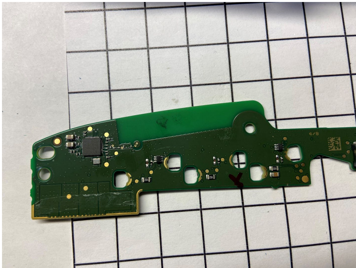
FDMHL6A Internal Photos
