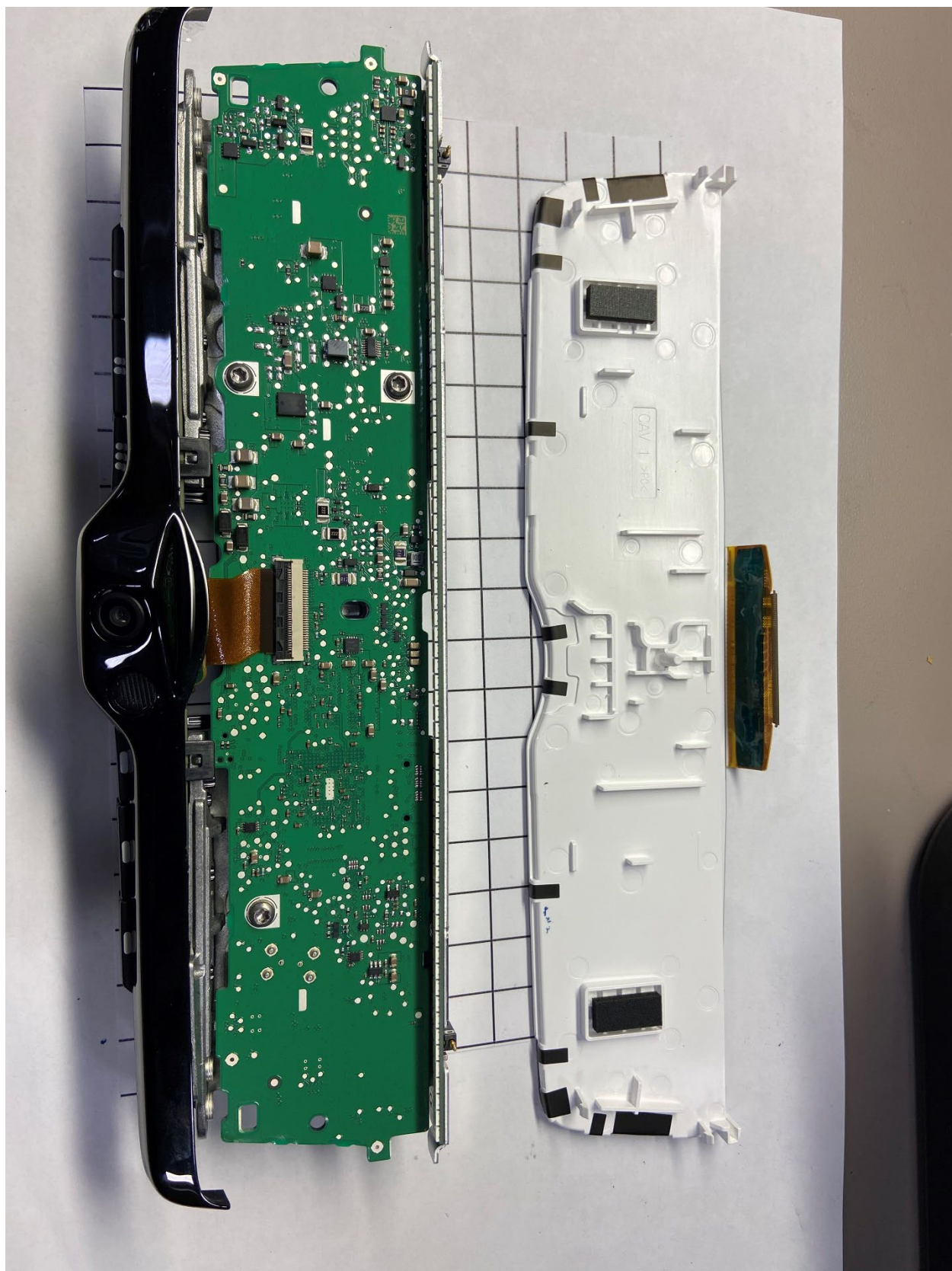
FDMHL6A Internal Photos
