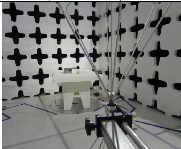
Bicon (30-200MHz) Setup Overview
