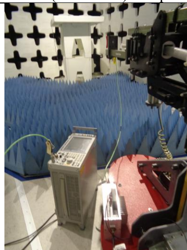
Bicon (30-200MHz) Setup Overview
