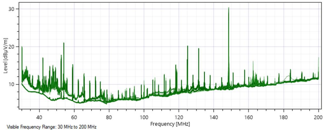
Emission Sweeps from 30MHz to 200MHz
