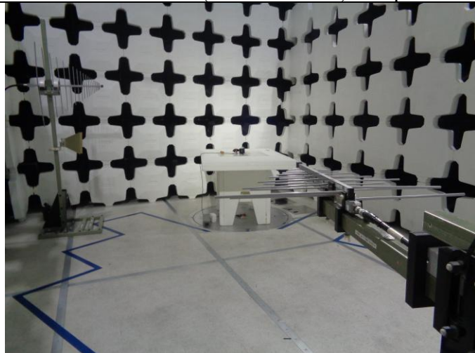
Class B Horn (1000-18000MHz) Setup
