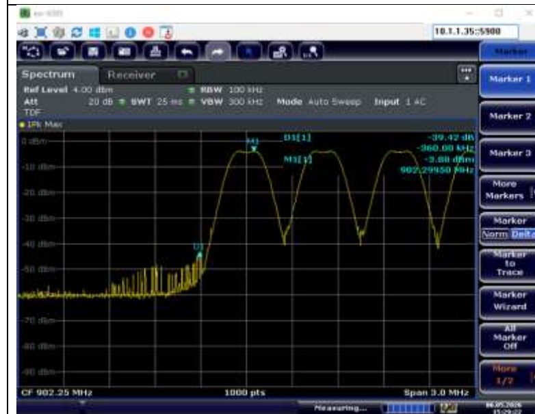
Hopping Low Frequency Band Edge
