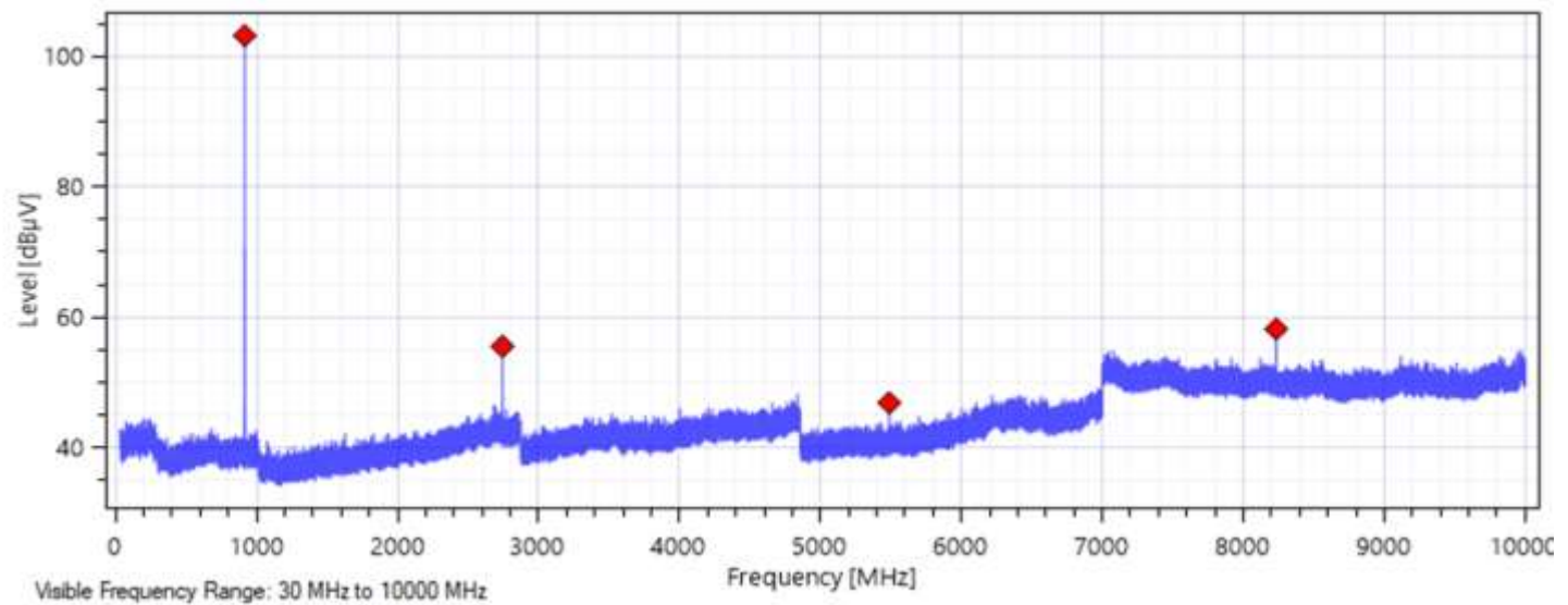
Trace: Mid Channel, Band: Band 5 (Peak Detector)
