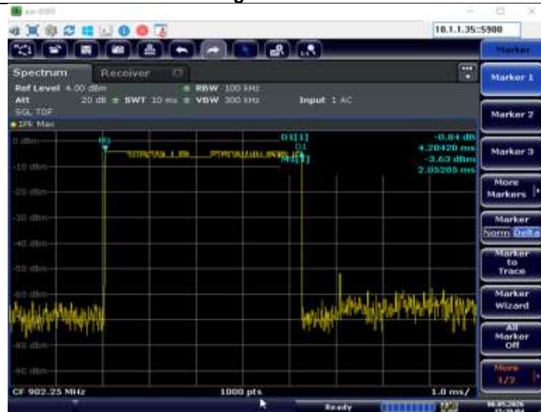
Dwell Time Low Band Measurement Plot for Wireless Diagnostics Mode
