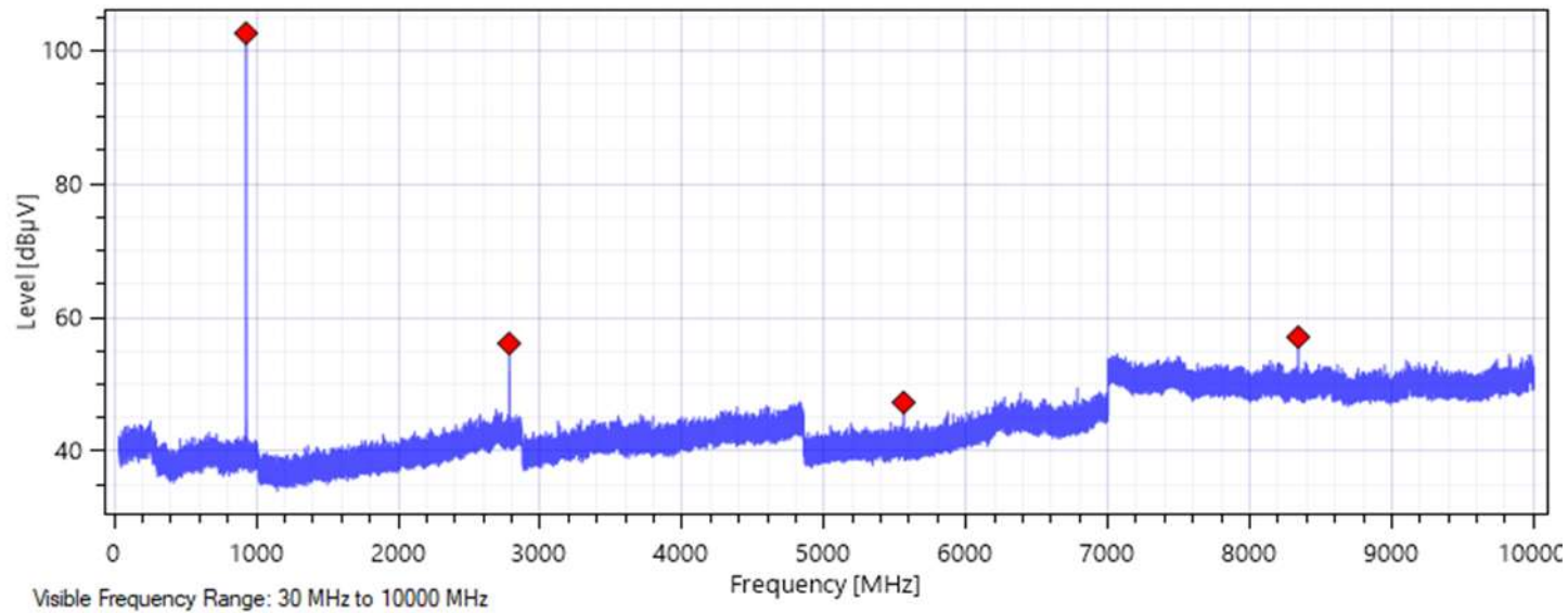
Trace: High Channel, Band: Band 5 (Peak Detector)
