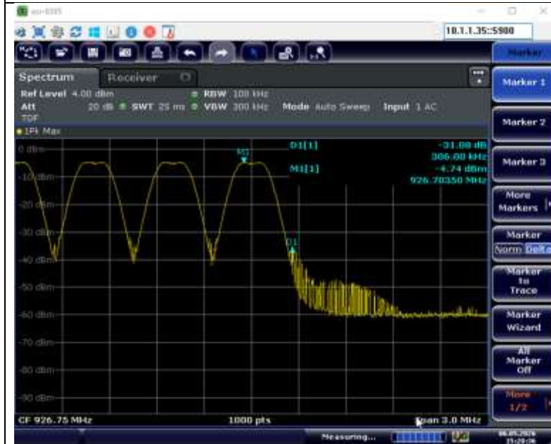
Hopping High Frequency Band Edge
