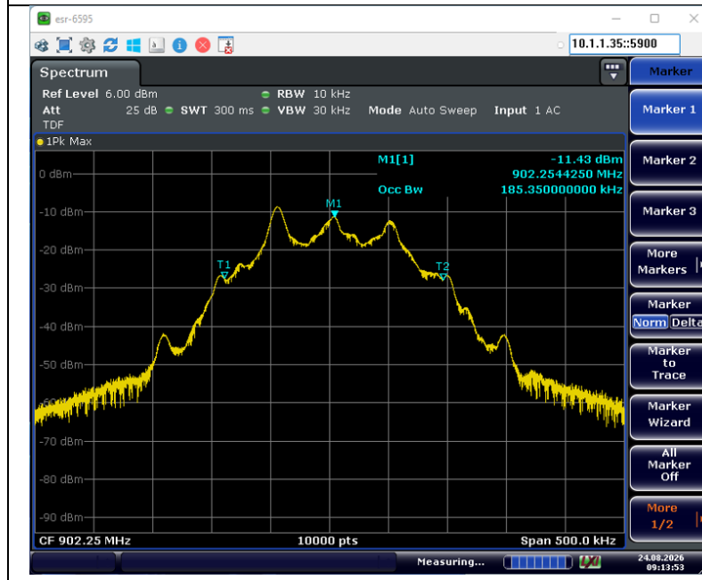
99% BW Low Band Measurement Plot
