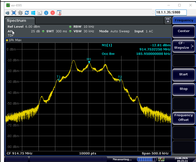
99% BW Mid Band Measurement Plot
