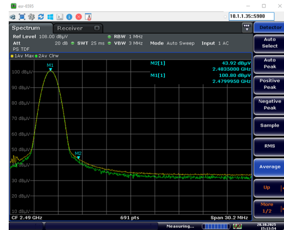
2480 MHz Average Horizontal
