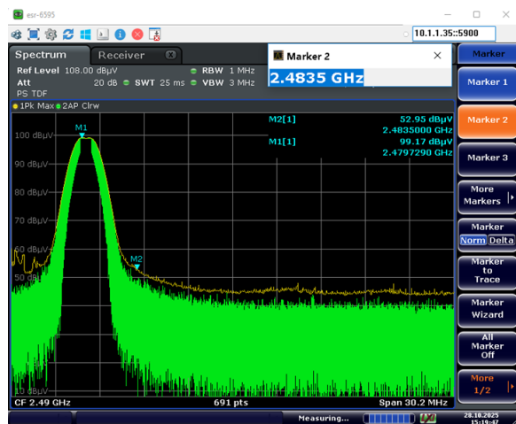
2480 MHz Peak Vertical
