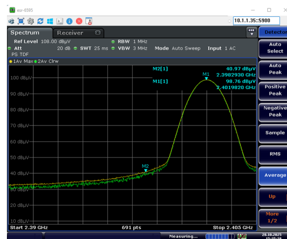
2402 MHz Average Horizontal
