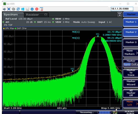
2402 MHz Peak Vertical
