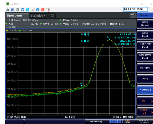
2402 MHz Average Vertical
