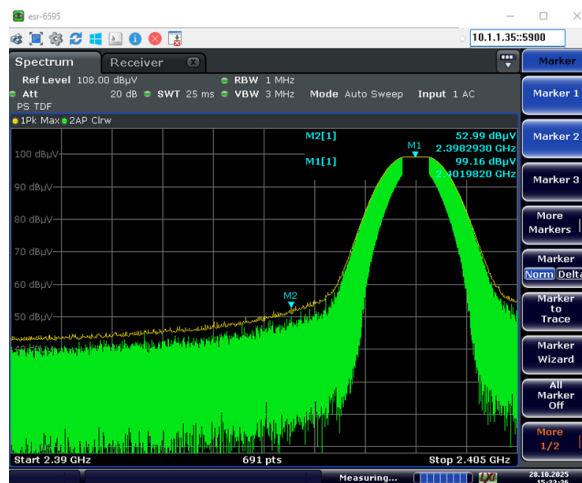
2402 MHz Peak Horizontal
