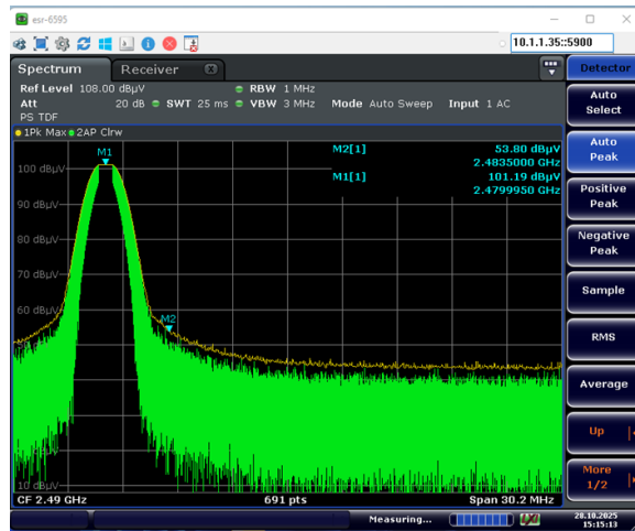
2480 MHz Peak Horizontal
