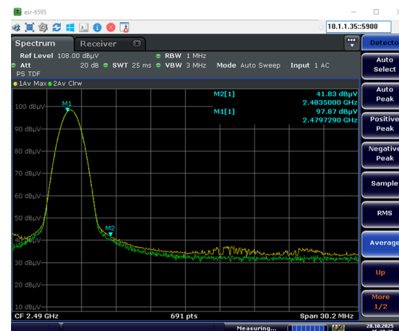
2480 MHz Average Vertical
