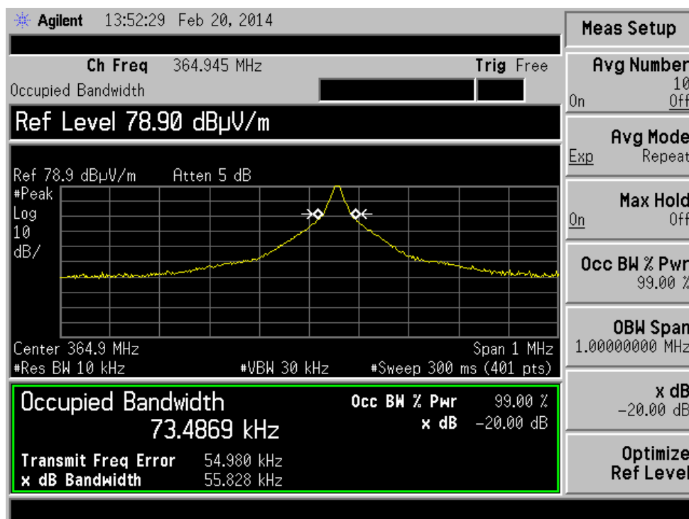
Measuring Occupied Bandwidth at -20dB points20
