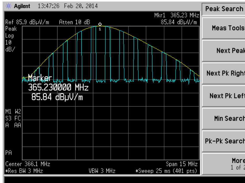
Measuring Peak Reference Level
