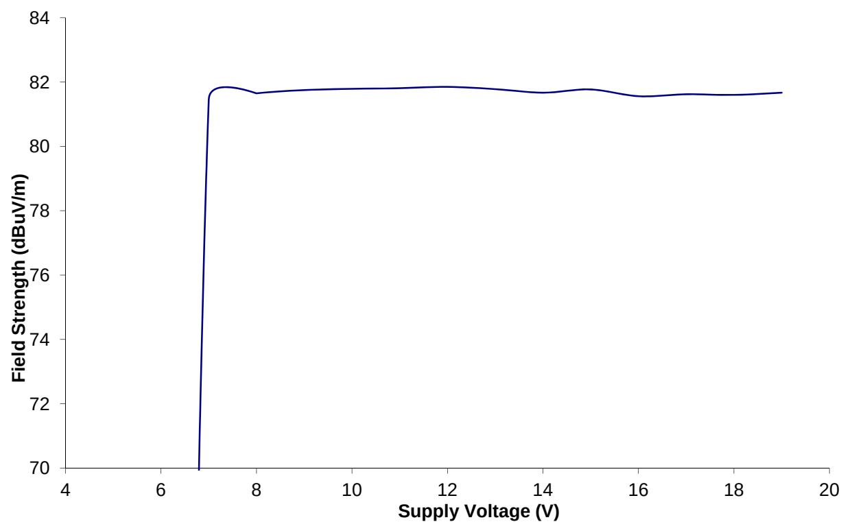
Output Field Strength vs. Supply Voltage
