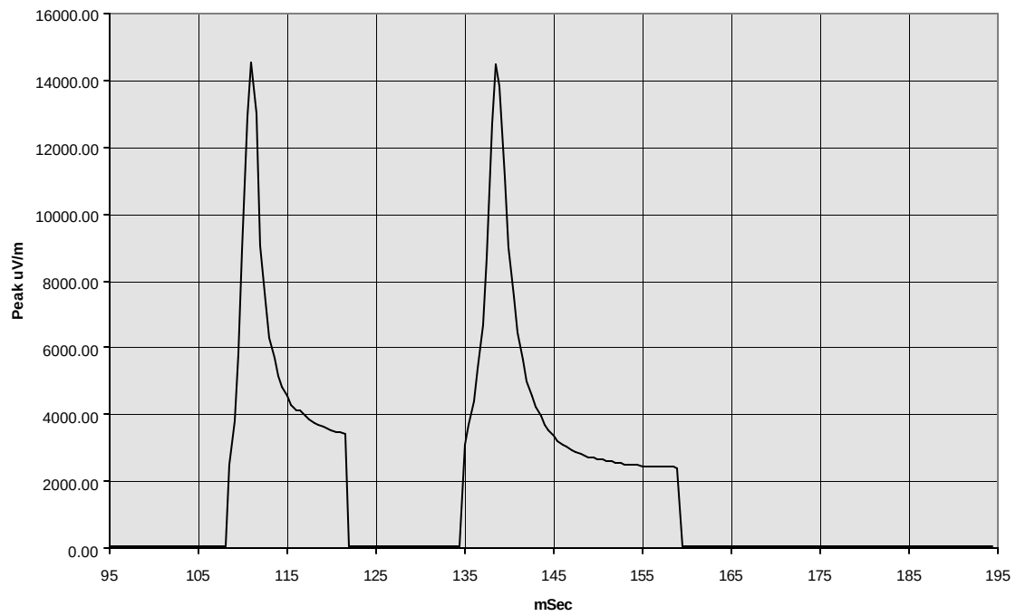
Coarse Tune Pulses, 310MHz fundamental Linear Scale
