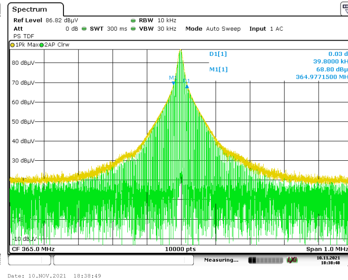
Measuring Occupied Bandwidth at -20dB points
