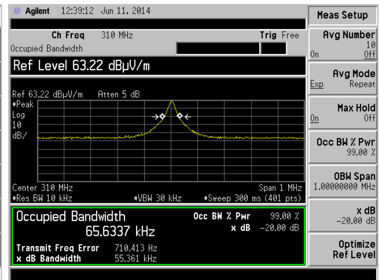
Measuring Occupied Bandwidth at -20dB points
