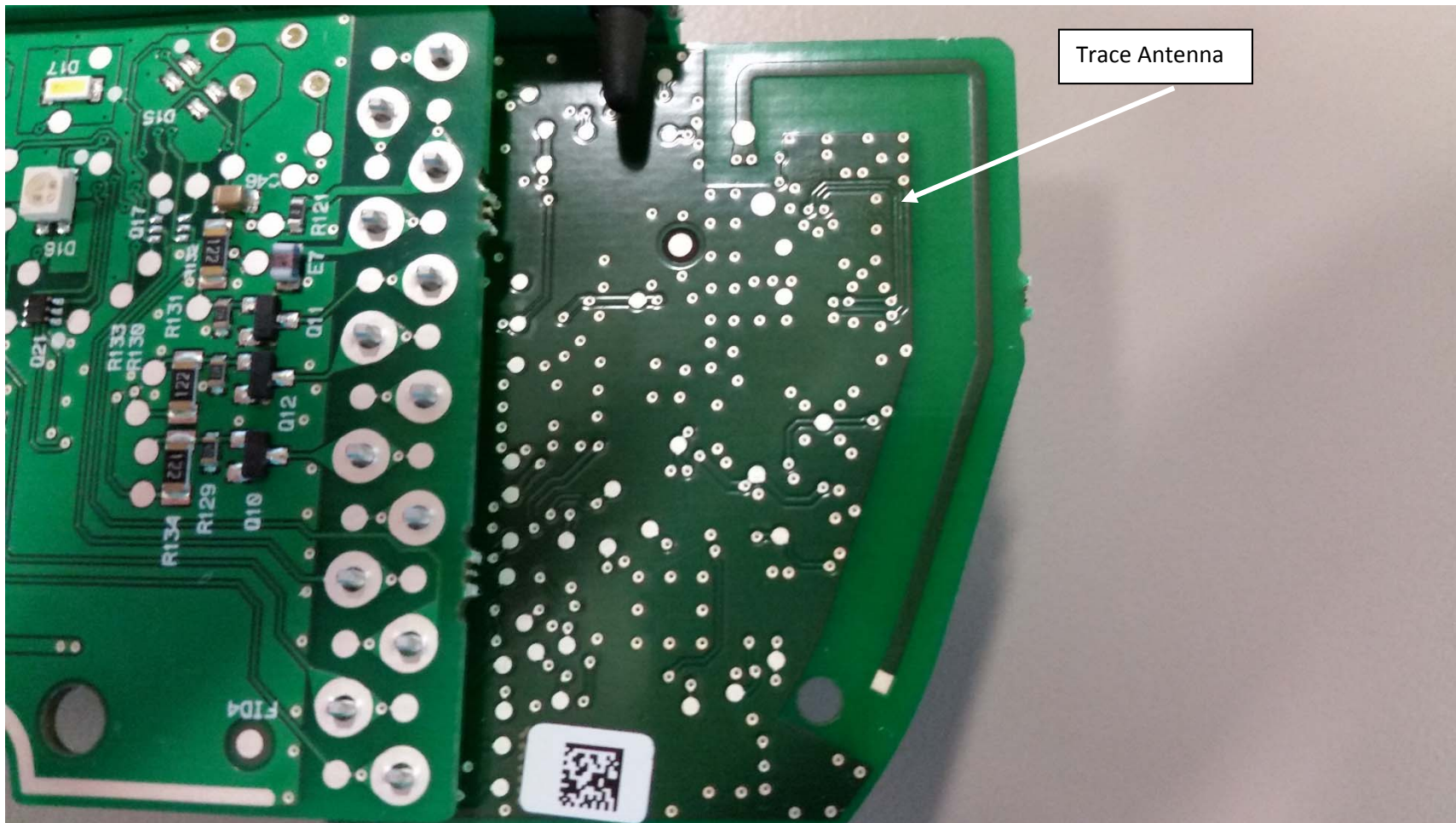
700-0599 – Transmitter Board
