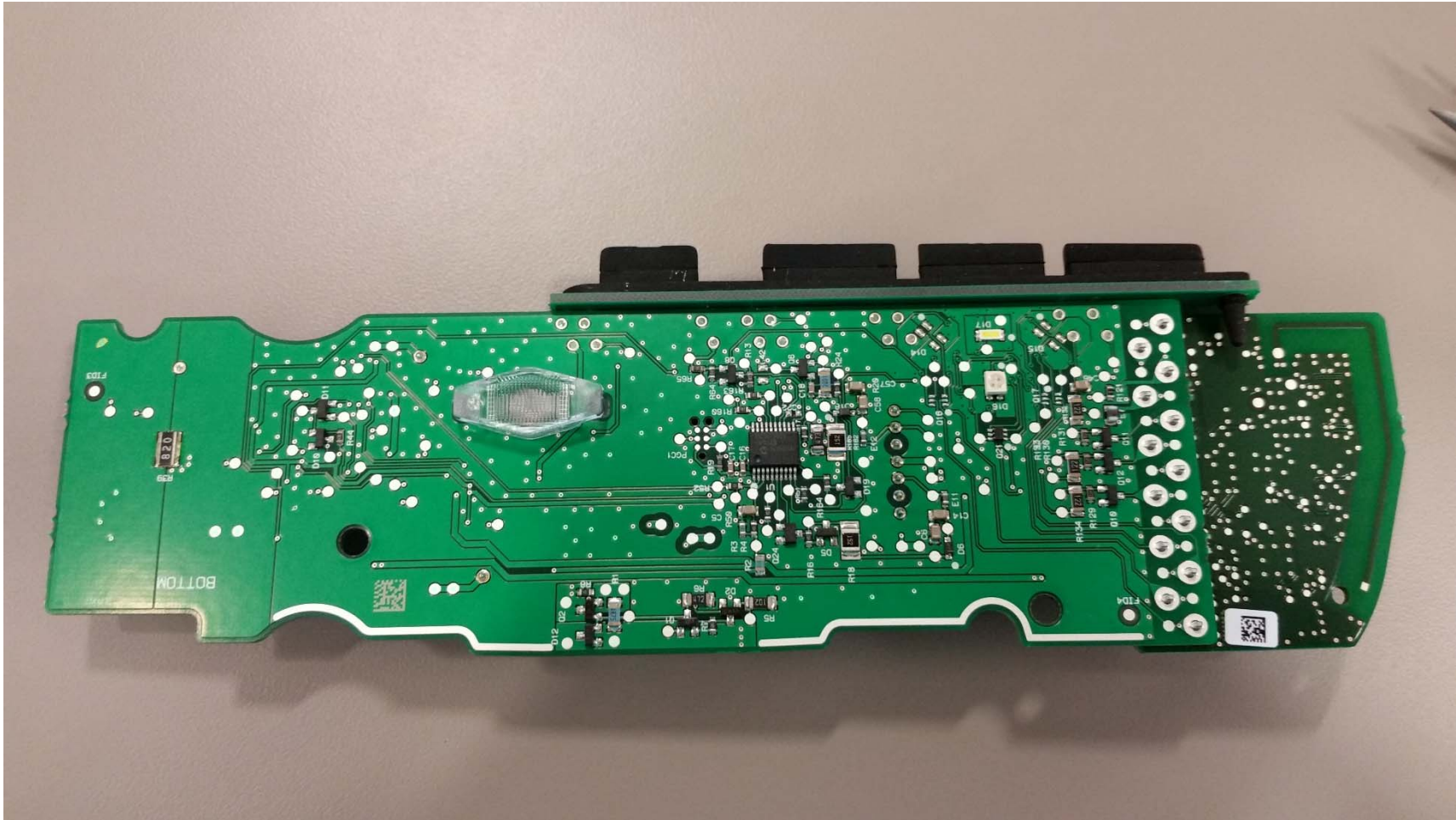
700-0583 – Mother Board
