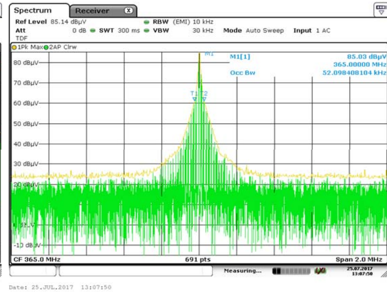
Measuring Occupied Bandwidth at -20dB points
