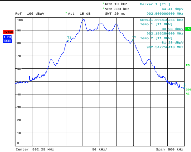
99% BW Low Band Measurement Plot
