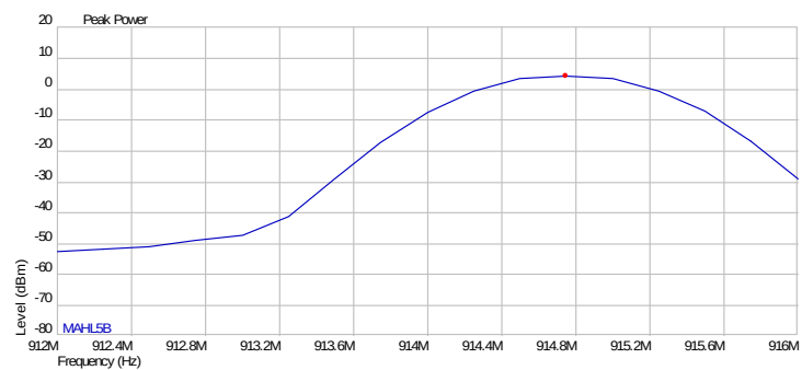
Peak Power Mid Band Measurement Plot
