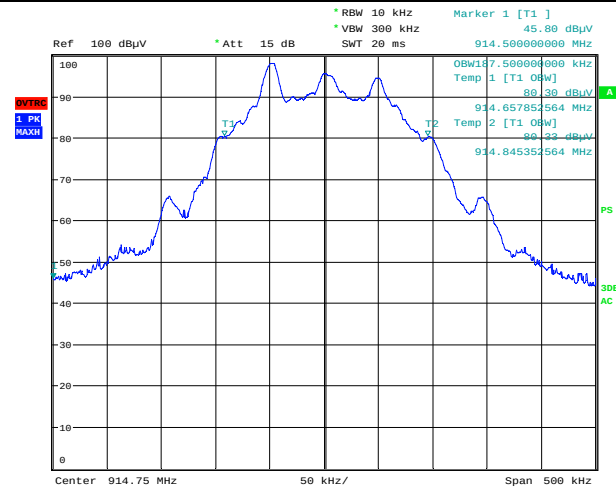
99% BW Mid Band Measurement Plot
