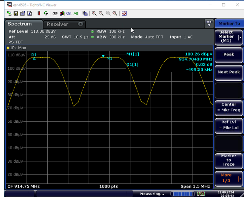
Channel Separation Mid Band Measurement Plot
