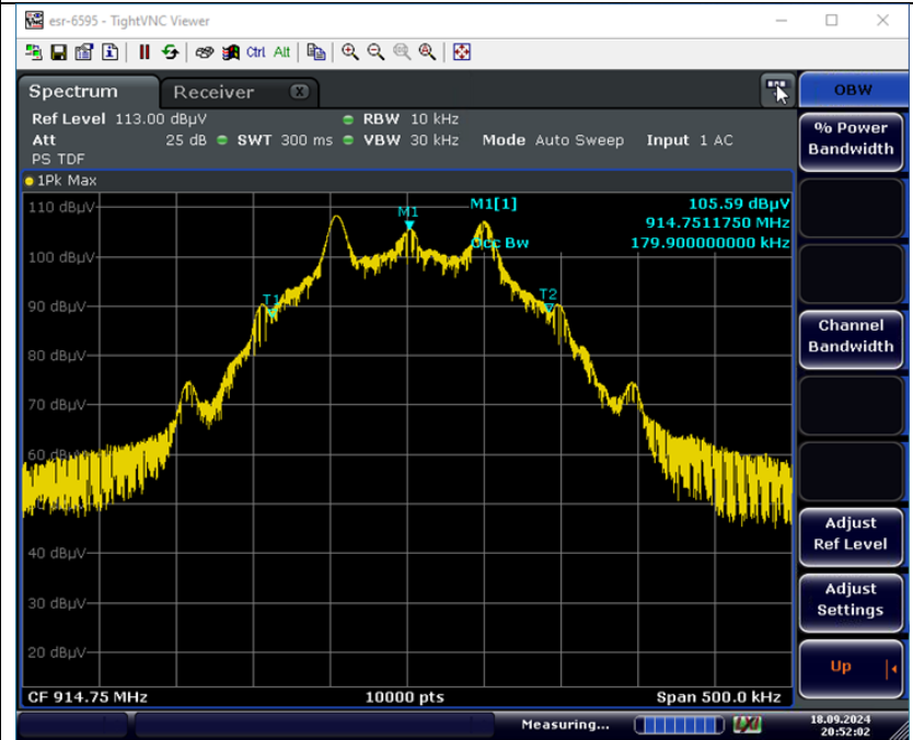
99% BW Mid Band Measurement Plot
