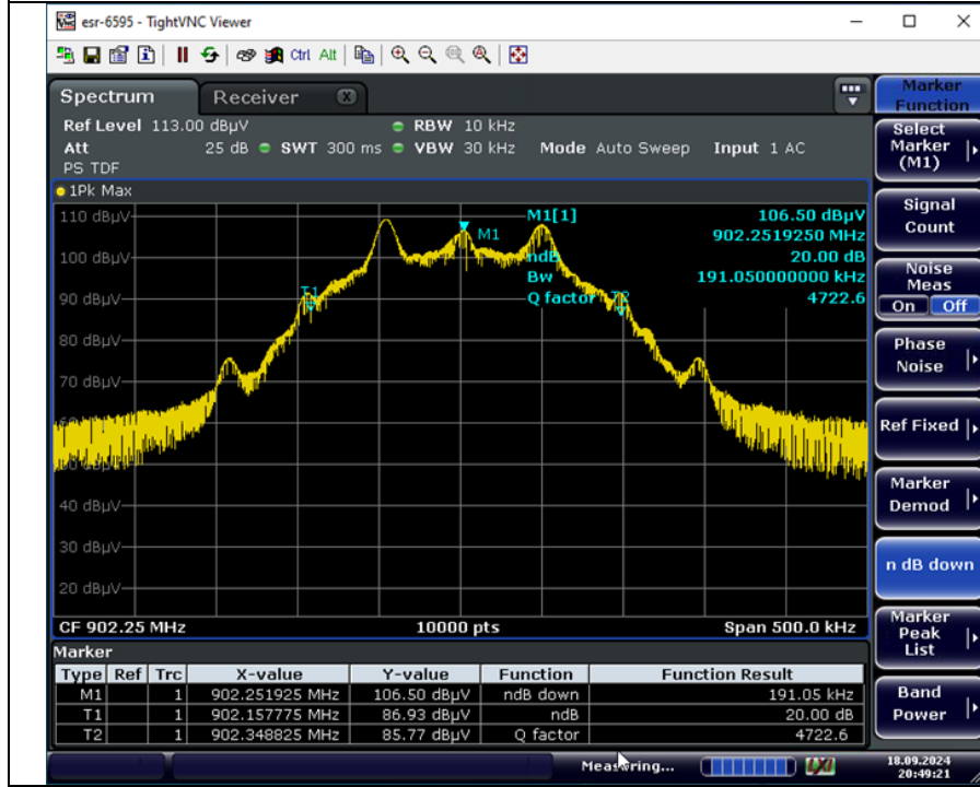
20 dB BW Low Band Measurement Plot
