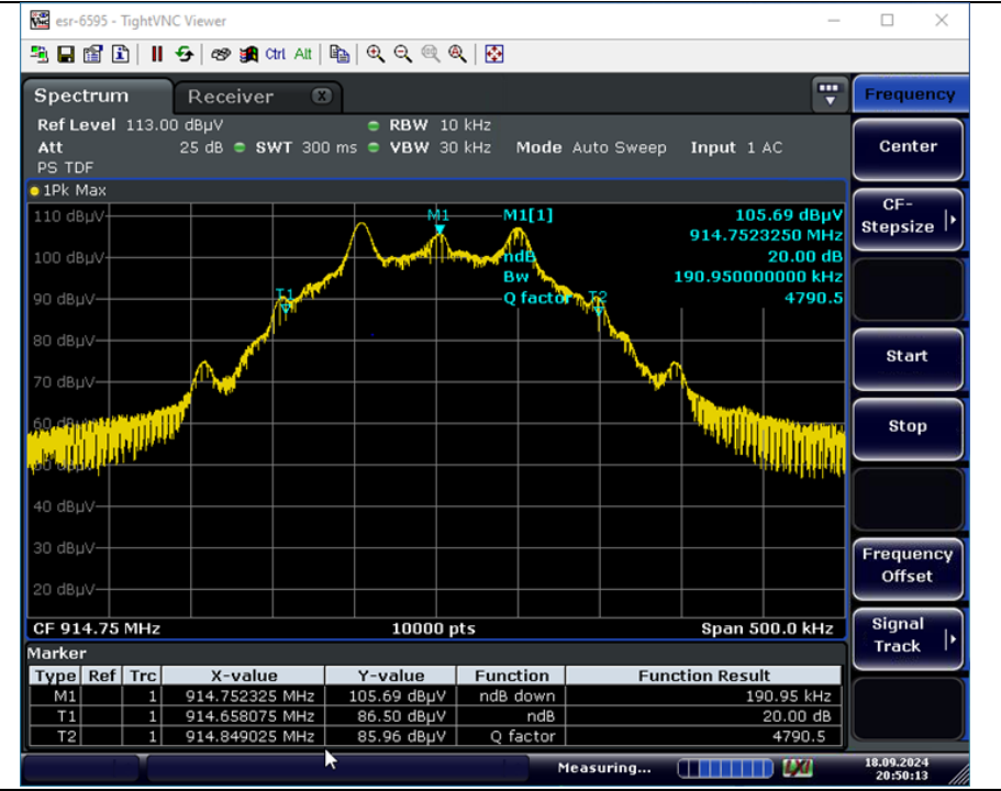
20 dB BW Mid Band Measurement Plot
