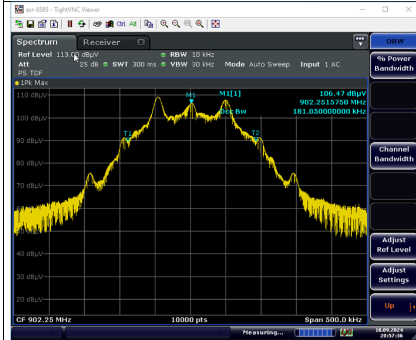
99% BW Low Band Measurement Plot
