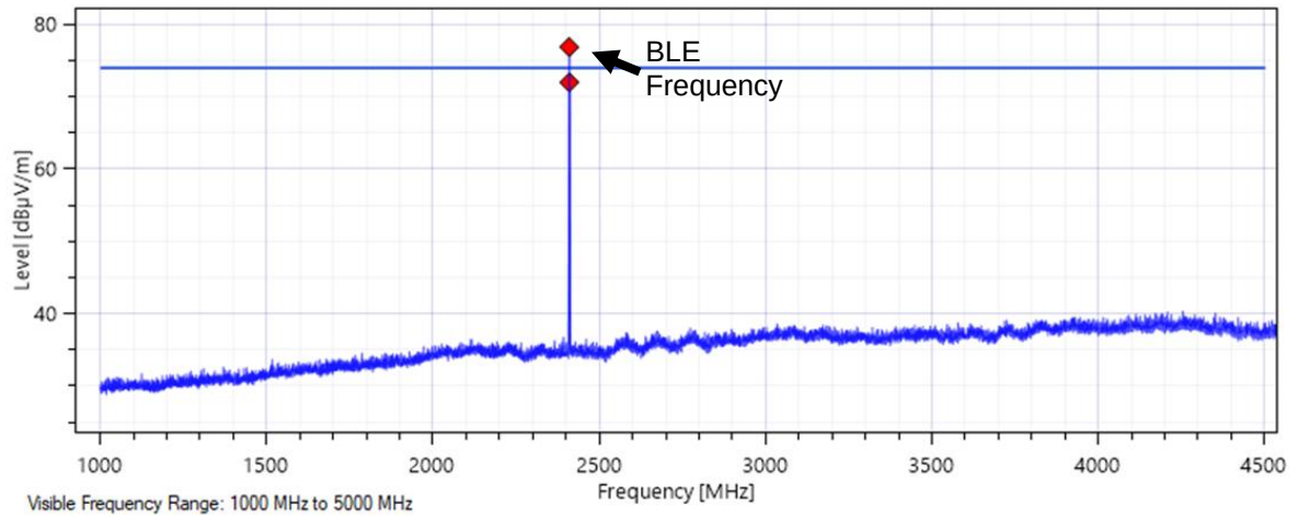
BLE 1000-4500 MHz Peak Vertical
