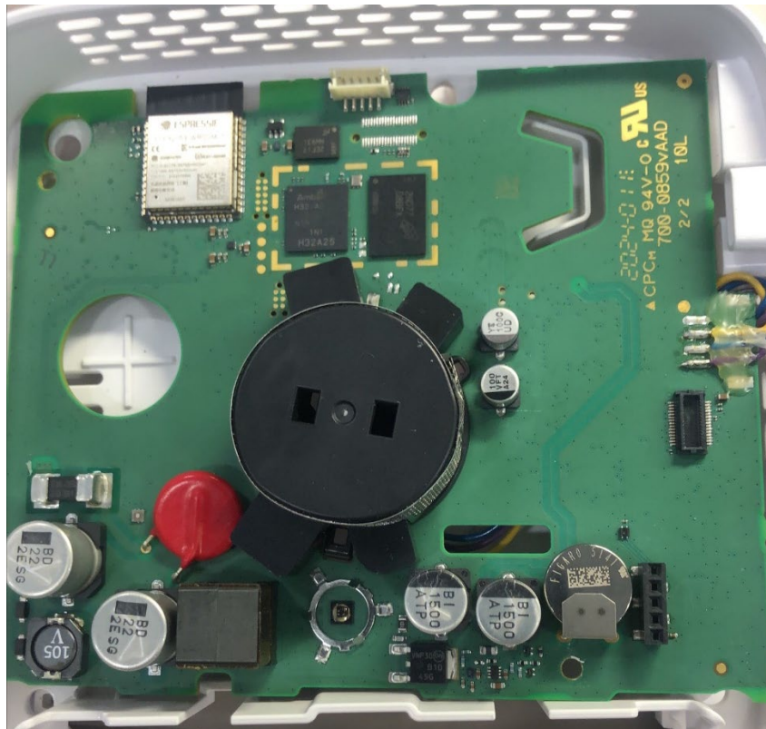
5.8 GHz Motion Sense Antenna Removed
