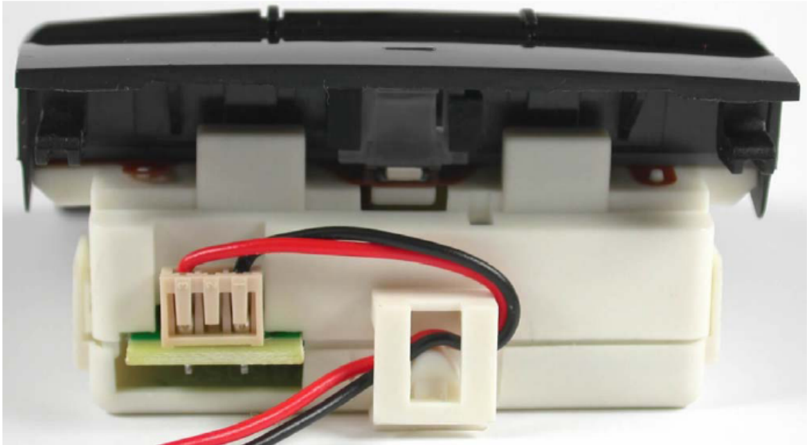
External photos side view
