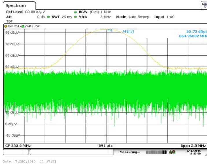
Measuring Peak Reference Level: 365MHz
