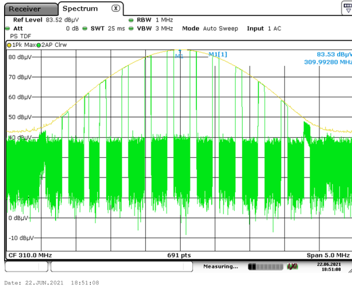
Measuring Peak Reference Level
