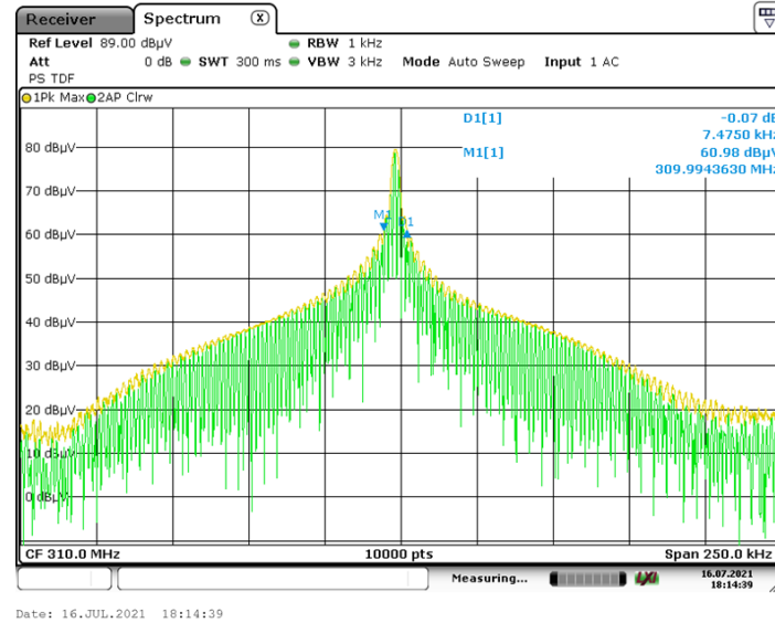
Measuring Occupied Bandwidth at -20dB points20
