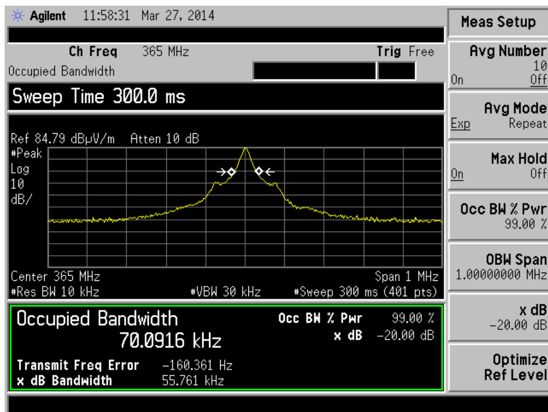
Measuring Occupied Bandwidth at -20dB points20
