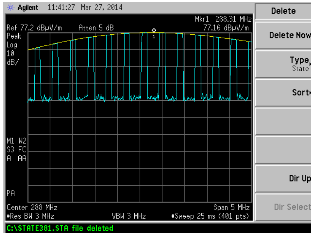
Measuring Peak Reference Level
