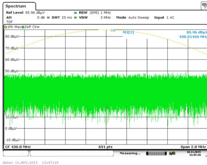
Measuring Peak Reference Level – 430MHz
