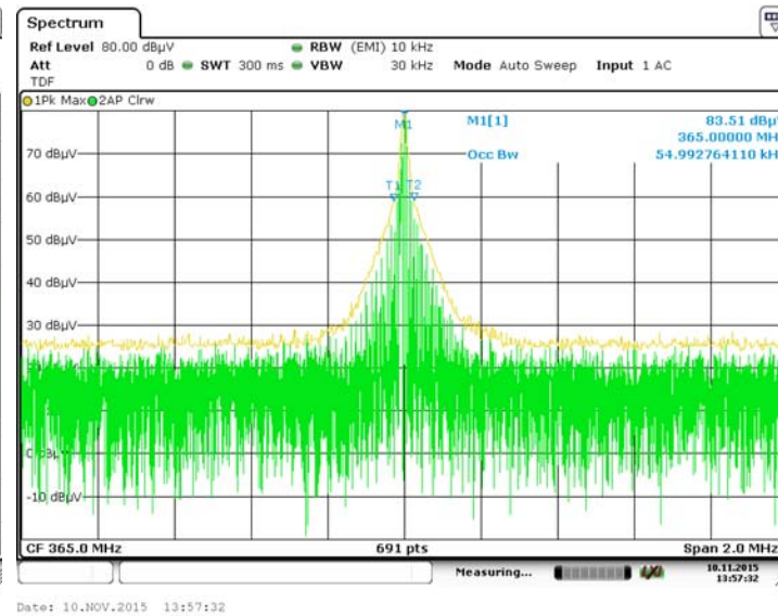
Measuring Occupied Bandwidth at -20dB – 365MHz
