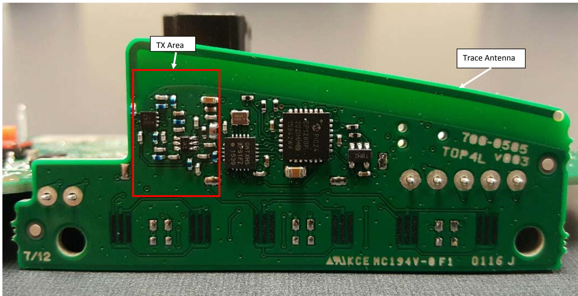
700-0585 – Transmitter Board
