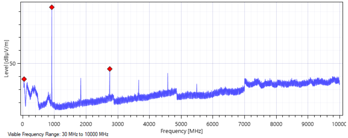
Trace: Mid Channel, Band: Band 5 (Peak Detector)
