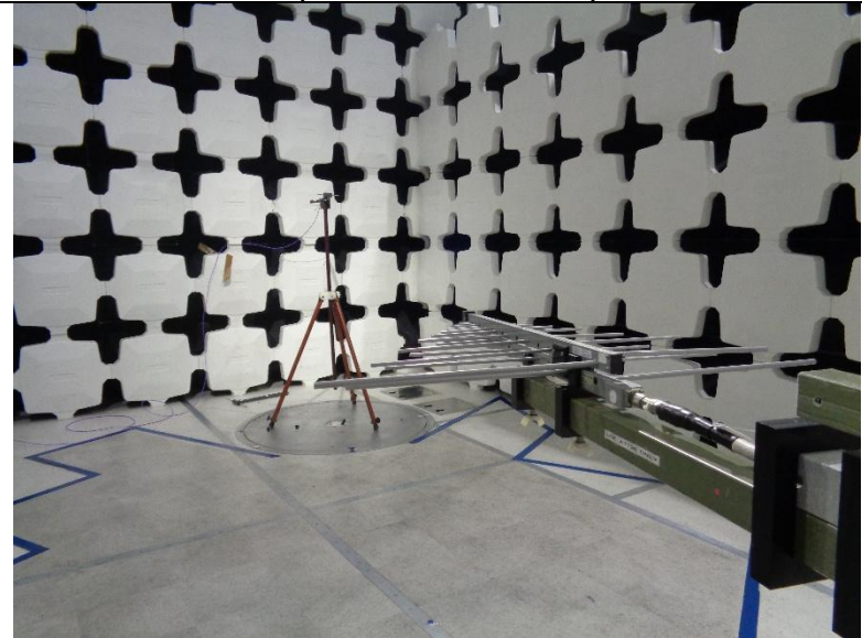
Dipole Antenna Setup
