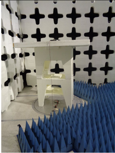
DUT Flat Orientation
