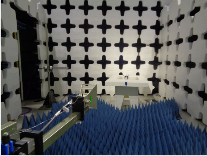
Class B Horn Antenna Setup
