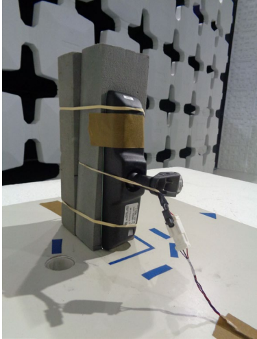
DUT End Orientation
