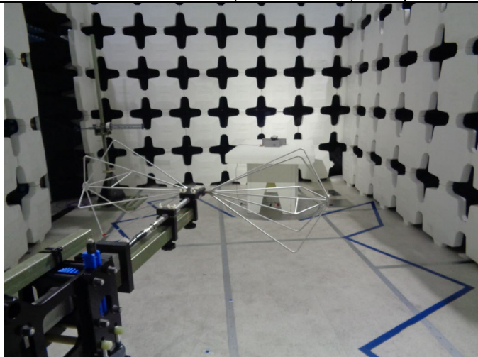
DUT Flat Orientation
