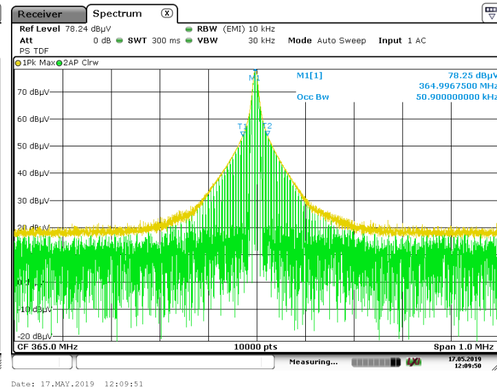
Measuring Occupied Bandwidth at -20dB points
