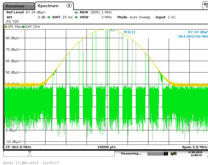
Measuring Peak Reference Level
