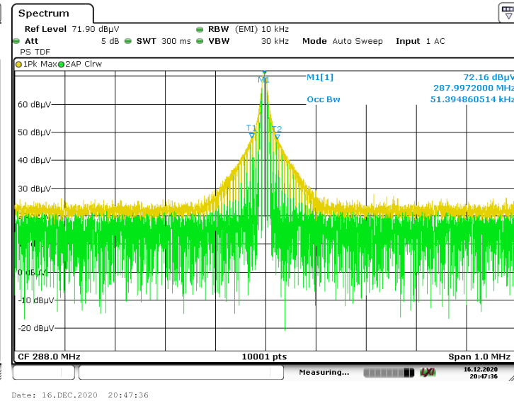
Measuring Occupied Bandwidth at -20dB points20
