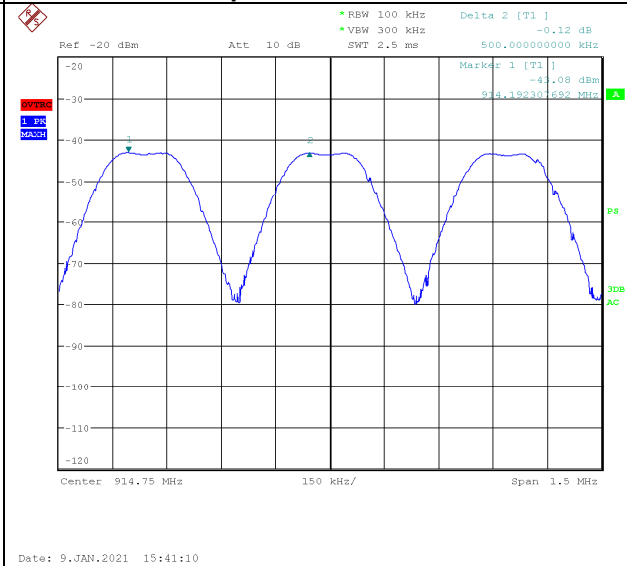
Channel Separation Mid Band Measurement Plot
