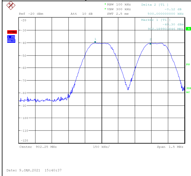
Channel Separation Low Band Measurement Plot
