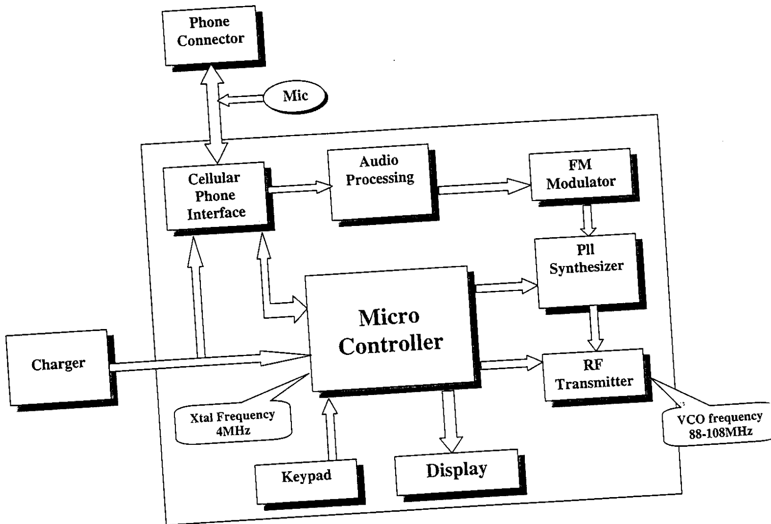
Cellular Phone Handsfree unit (FM) Block Diagram
