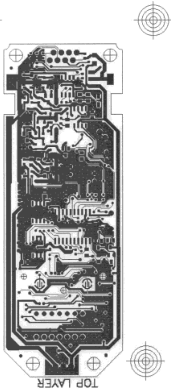
Figure No.1 Cell-man printed circuit board
