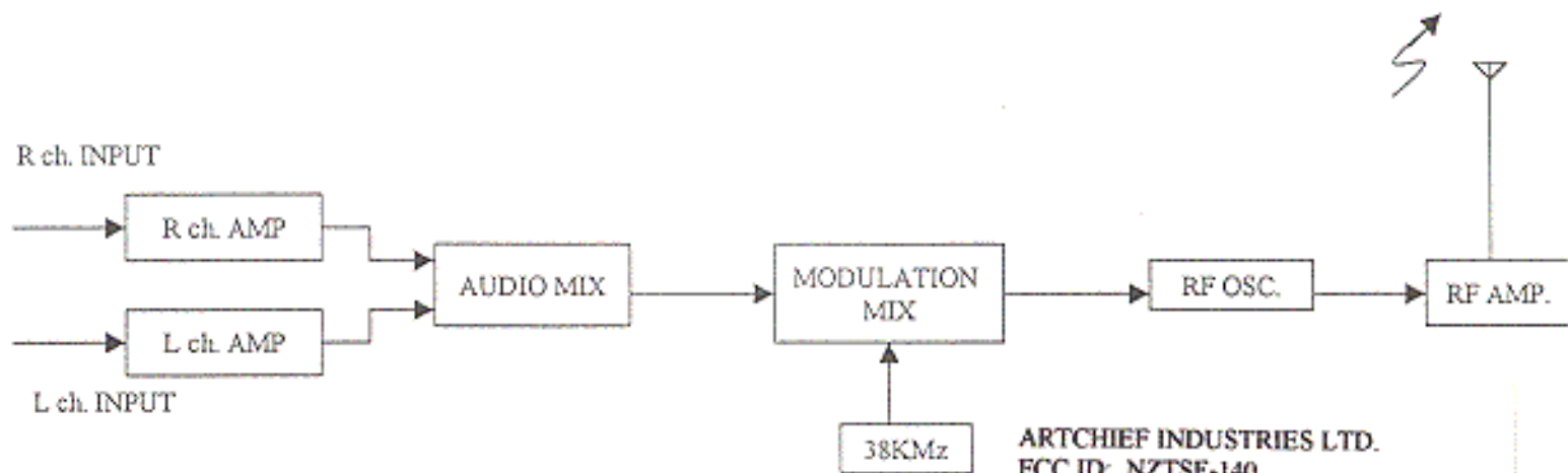
SF-140 BLOCK DIAGRAM
