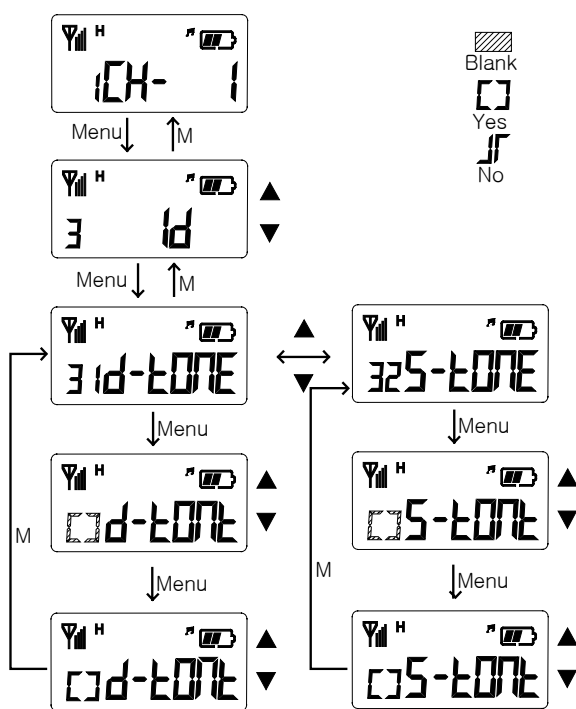
Figure 5.14 ID ANI
