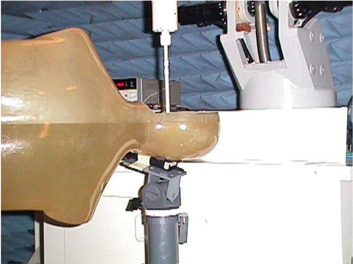
< Head Right Ear SAR Measurement - Overview >
