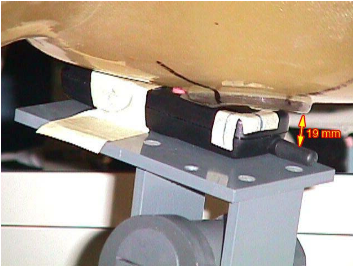
< Head Right Ear SAR Measurement – Close-Up View >
