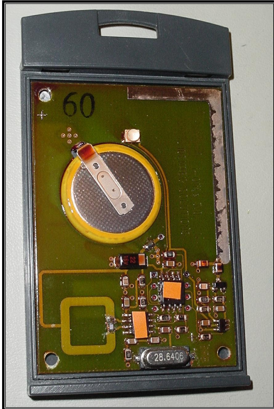
PHOTOGRAPH 8: i-D2 NA PCB IN CASE
