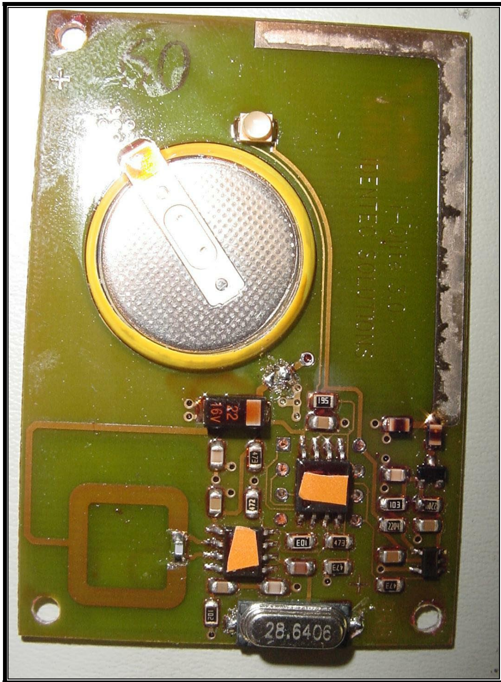
PHOTOGRAPH 9: i-D2 NA CIRCUIT CARD TOP
