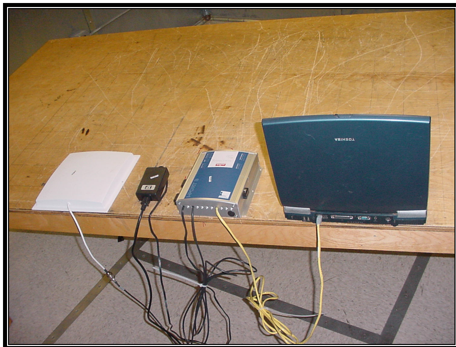
PHOTOGRAPH 11: CONDUCTED EMISSIONS TEST CONFIGURATION - PATCH ANTENNA BACK VIEW
