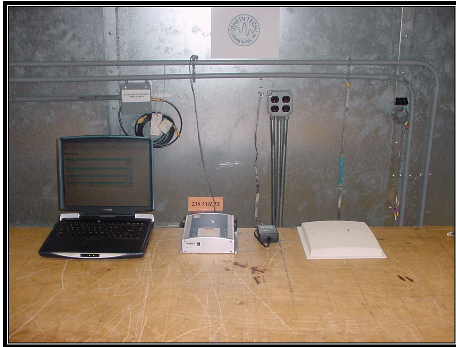
PHOTOGRAPH 10: CONDUCTED EMISSIONS TEST CONFIGURATION - PATCH ANTENNA FRONT VIEW
