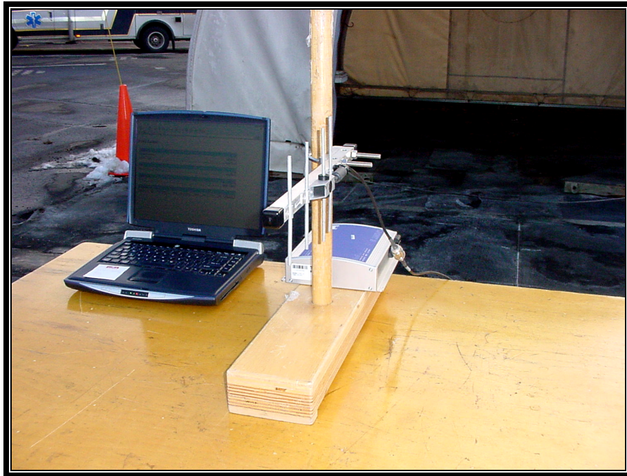
PHOTOGRAPH 6: RADIATED EMISSIONS TEST CONFIGURATION - YAGI ANTENNA FRONT VIEW
