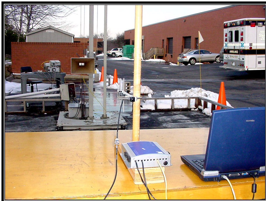
PHOTOGRAPH 7: RADIATED EMISSIONS TEST CONFIGURATION - YAGI ANTENNA REAR VIEW
