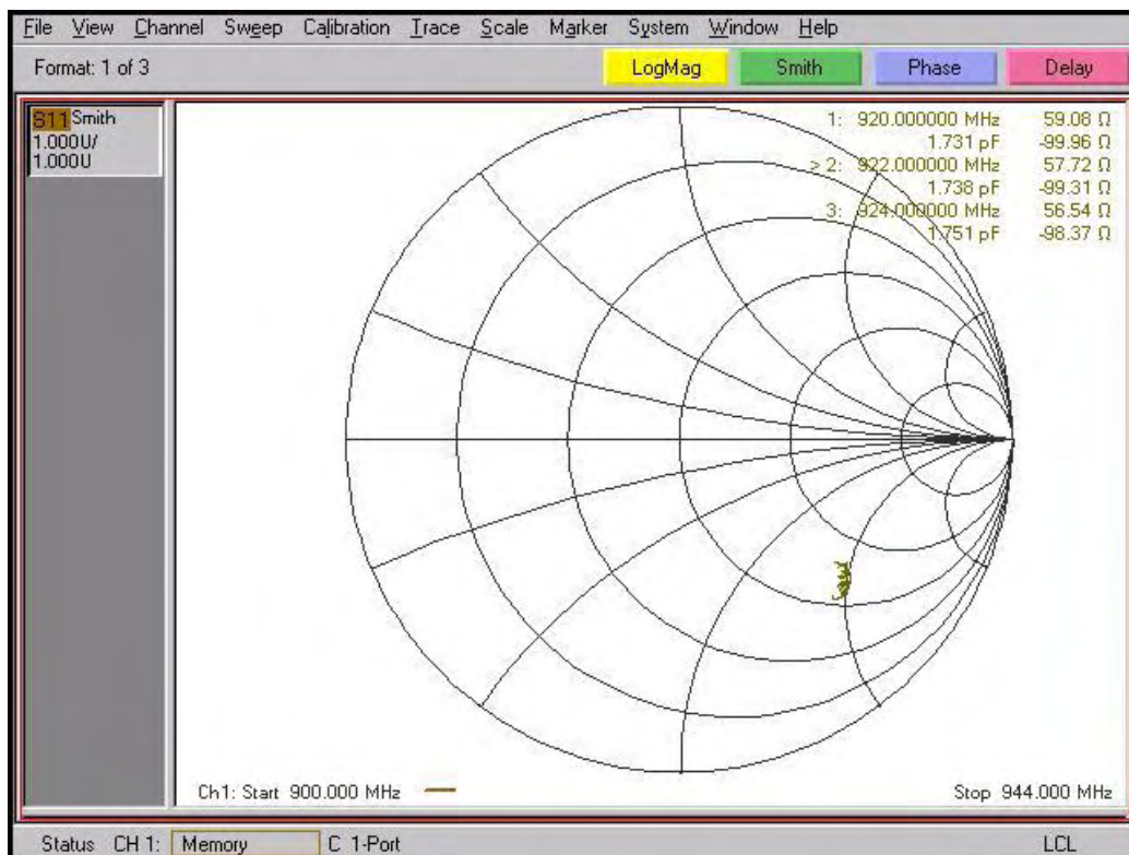
Fig 2. Smith Chart
