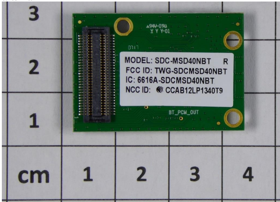
WLAN module and antenna
