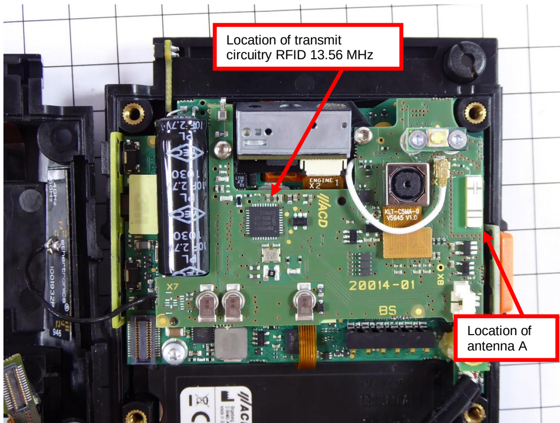
Location of transmit circuitry and antennas:
