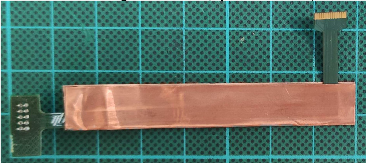
80014340 ACD M2Smart_ACD SE contact board plug-in module Siemens – top view
