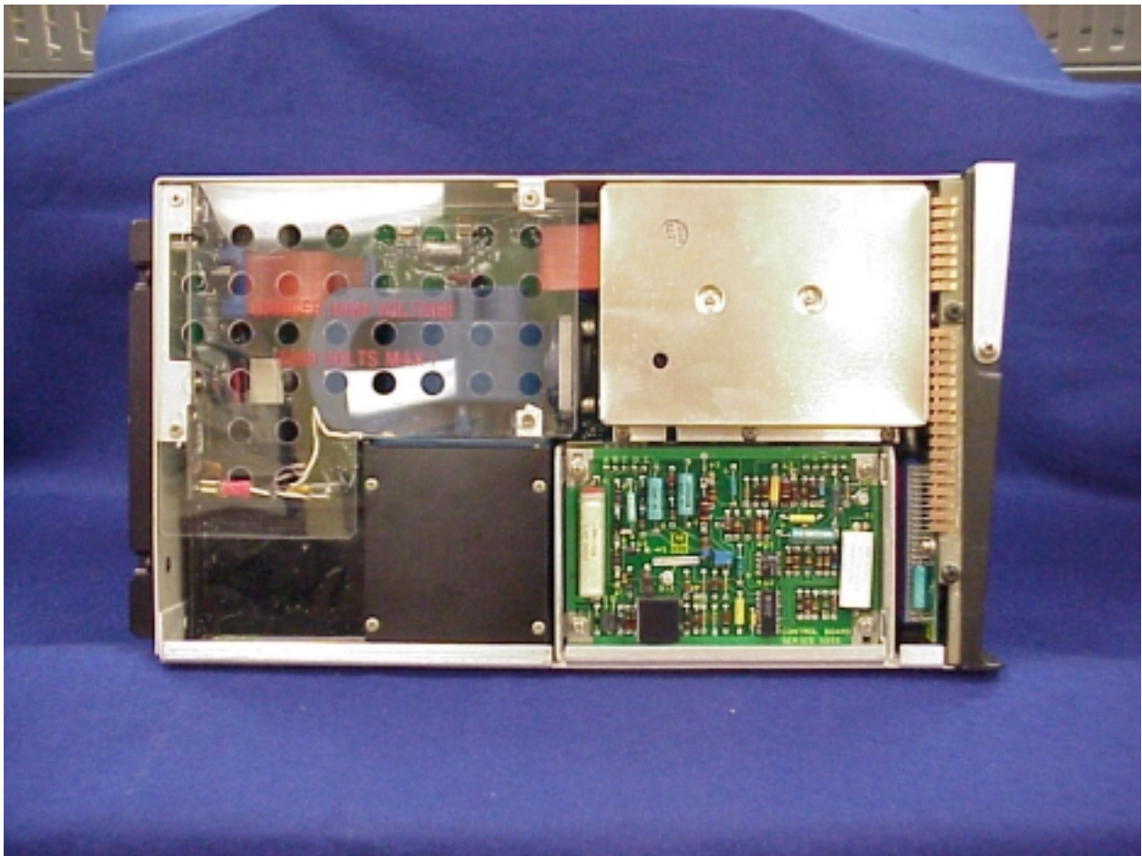
Figure 3 RT1401 Left Side Internal.JPG
