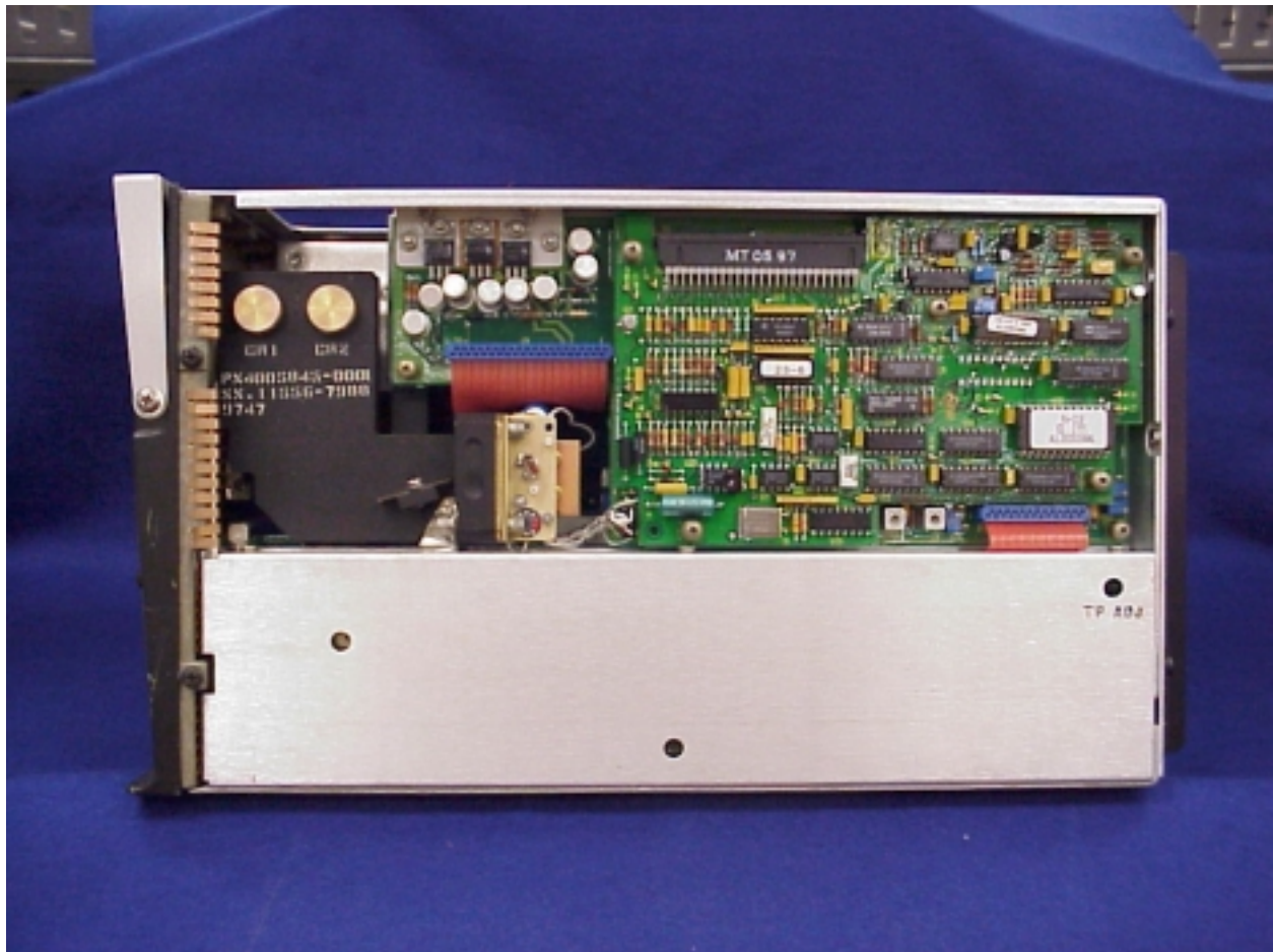
Figure 4 RT1401 Right Side InternalJPG
