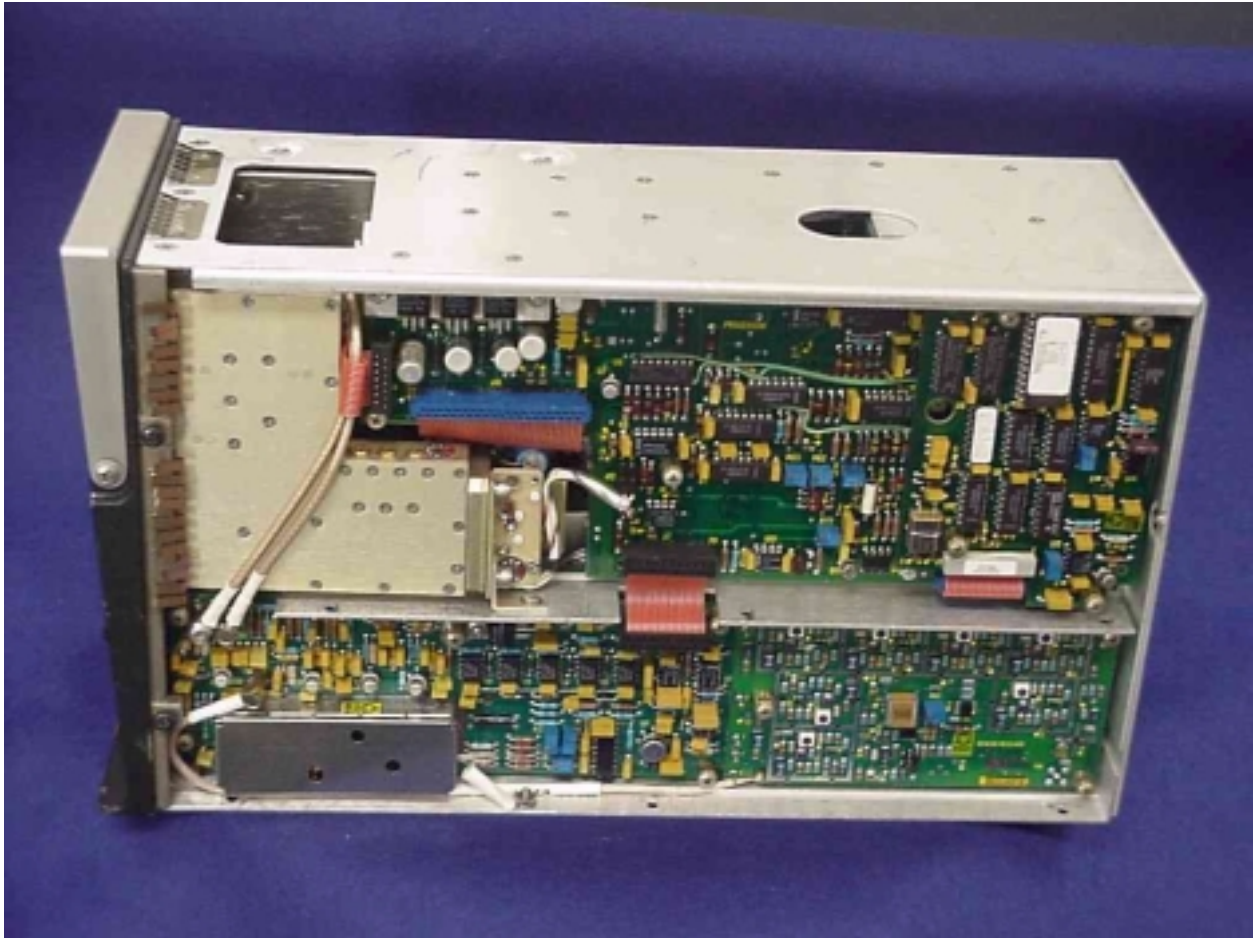
Figure 4 RT-1501A, Right Side With Cover Off.JPG
