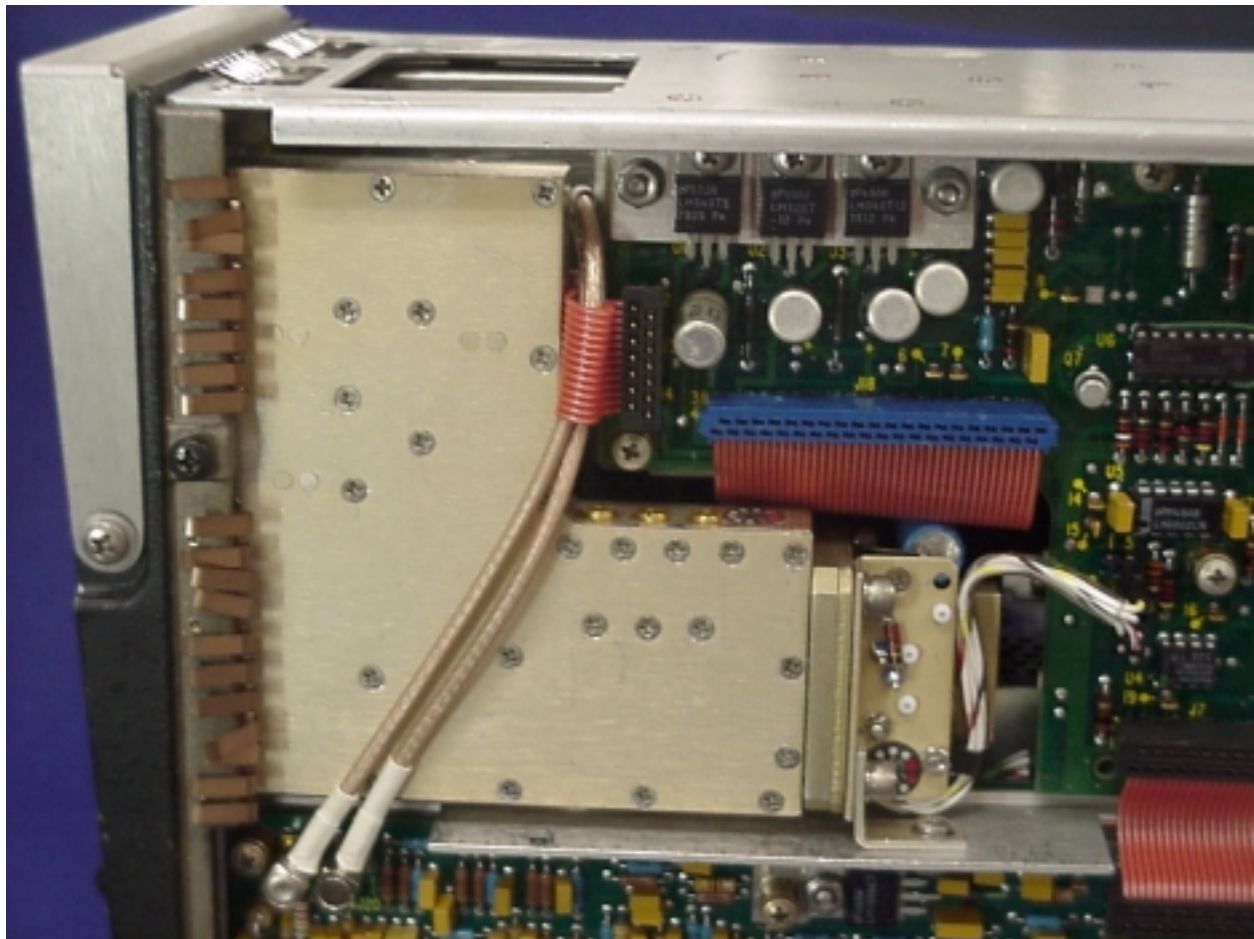
Figure 5 RT-1501A, Pre-Amp Limiter Closeup.JPG
