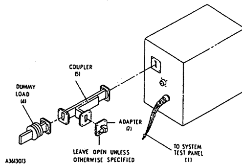
RT-1501A System Test Setup Figure 4-2
