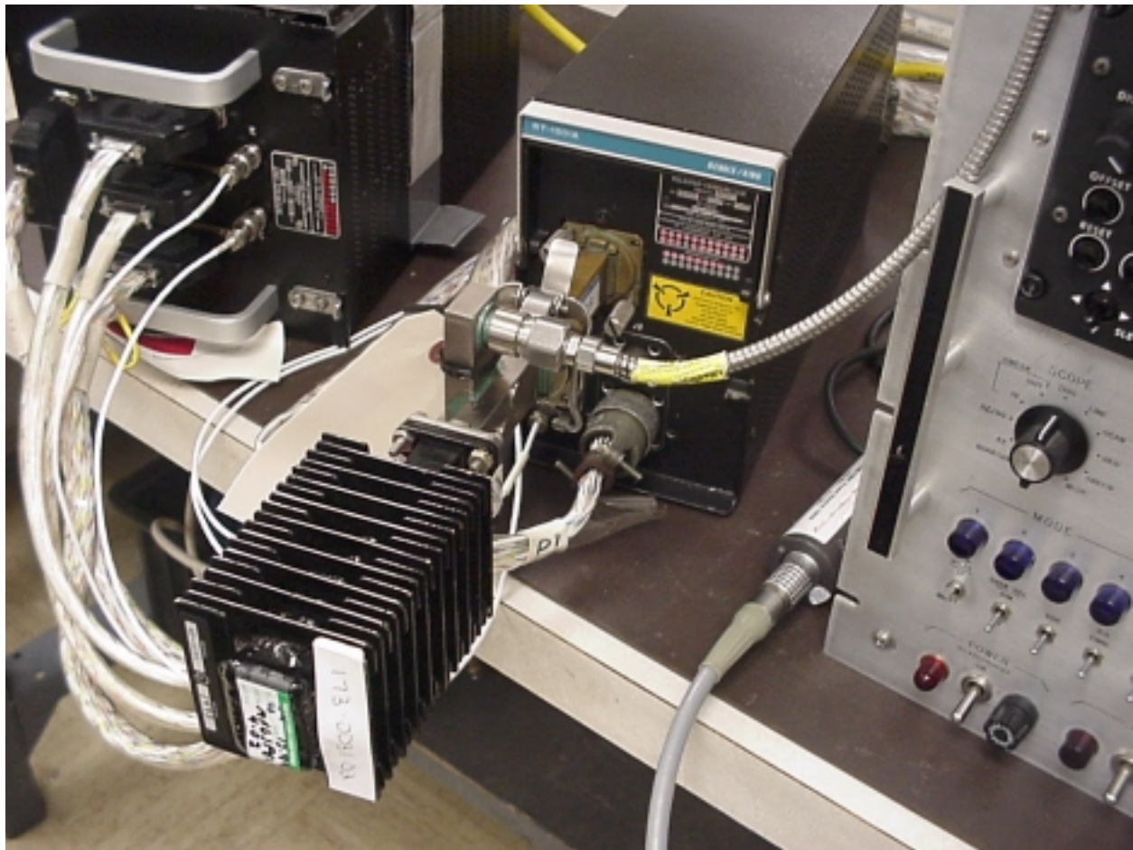
Figure 3 RT-1501A, With load.JPG
