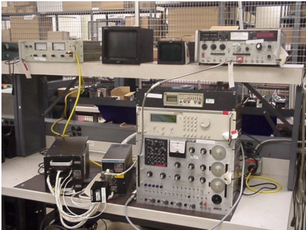
Figure 1 Test Setup, Full View.JPG
